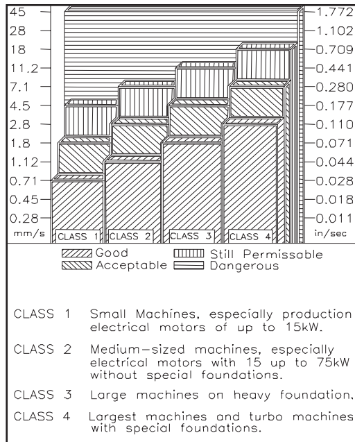
Vibration Severity Chart
